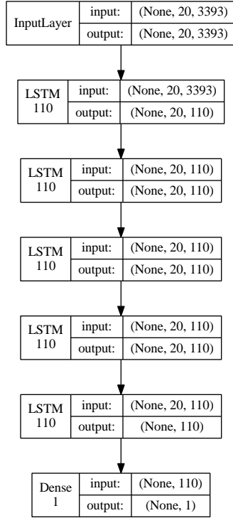
Figure 22. LSTM architecture
