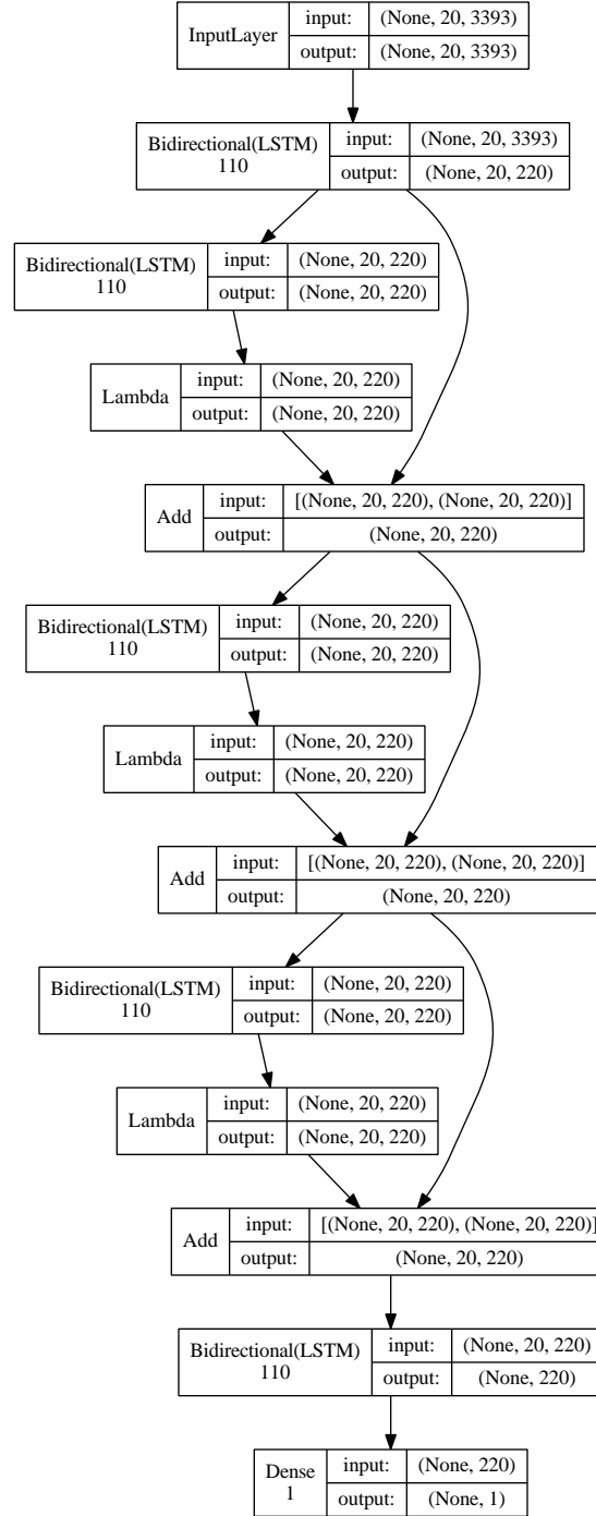
Figure 24. BDRLSTM architecture
