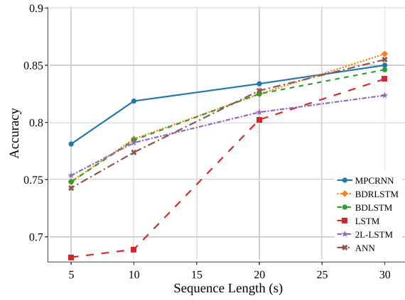
(b) Optimal-Stopping Validation-Set Group Model
