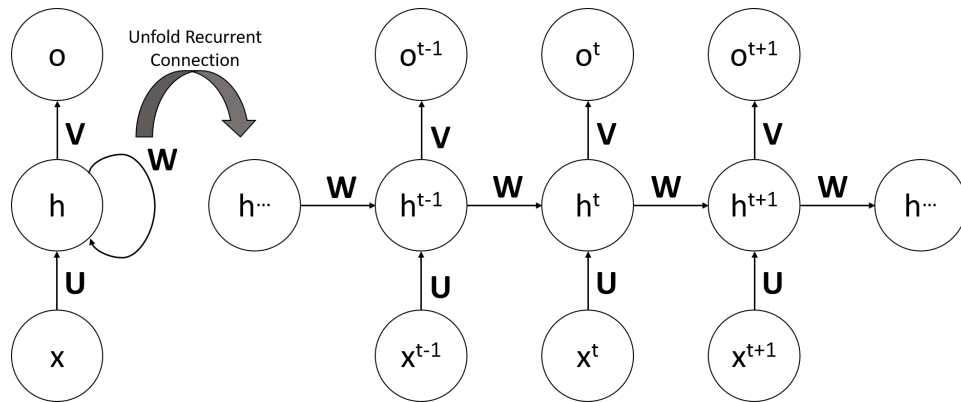
Figure 3. Temporal unfolding of the recurrent unit in the computational graph. On the left side is the cyclic graph. All cycles have been removed from the graph on the right side by unfolding the cyclic graph in time. Note the weight matrices U , V , and W are shared across time.
